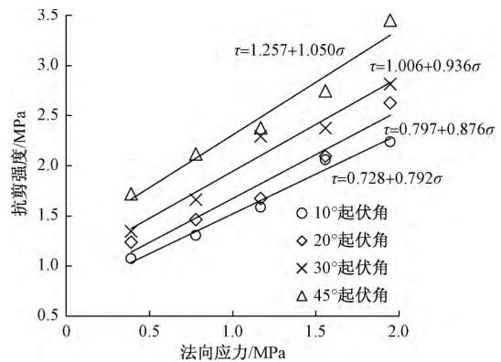
图 9 结构面在不同起伏角度下的 \tau - \sigma 关系图 Fig. 9 Relationship between the shear strength and normal stress of the structural plane at different asperity inclination angles
